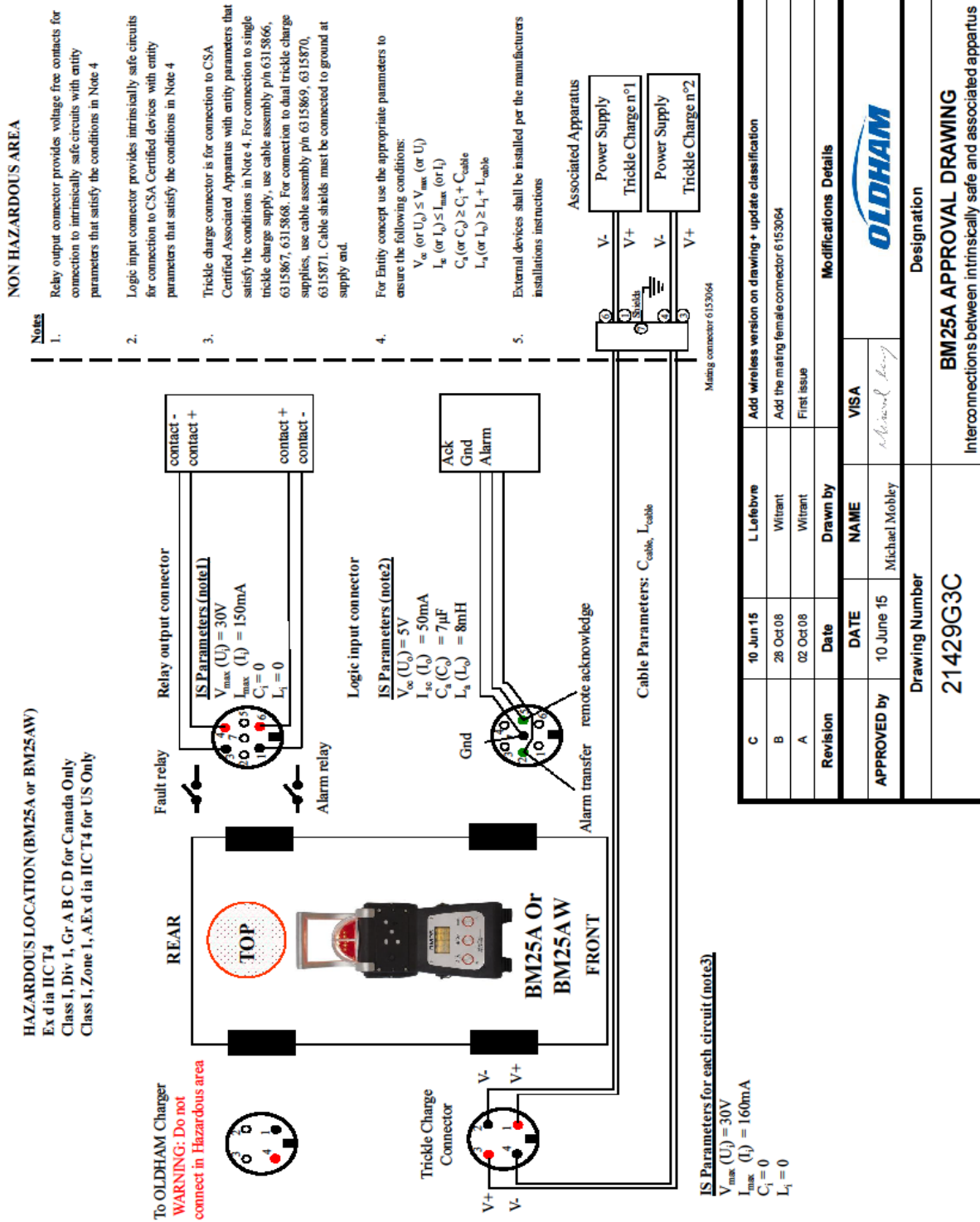
Figure 47 : Control Drawing for BM 25A/AW Connections
